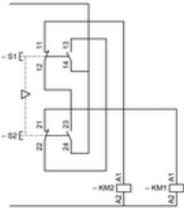
Control of 2-Speed Reversing Motor With XESD1281
