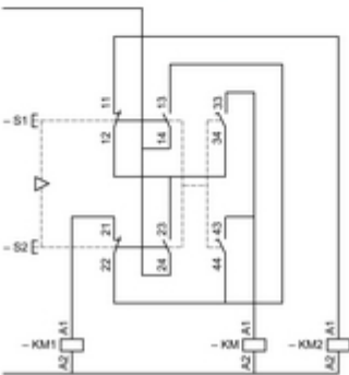
Control of 2-Speed Reversing Motor With XESD1281
